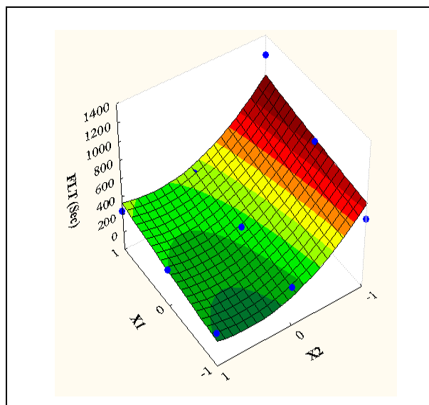
Figure 10: Response surface plot for FLT (sec)
