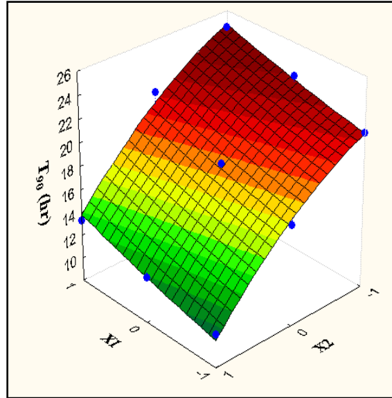
Figure 8: Response surface plot for t_{90} Full and reduced model for Q_{12} (%)
