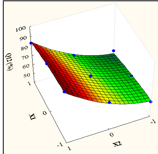
Figure 9: Response surface plot for Q 12
