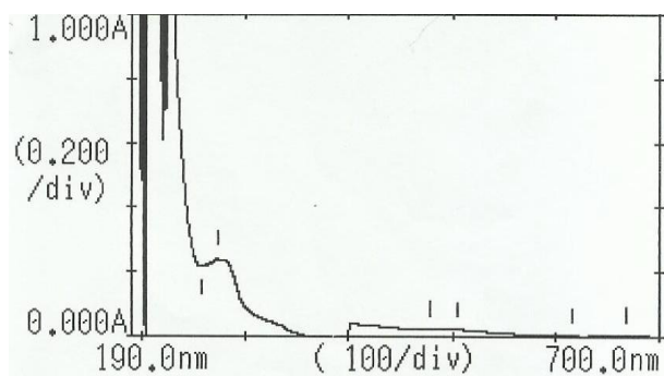
Fig.4: The sodium acetate spectrum of compound I
