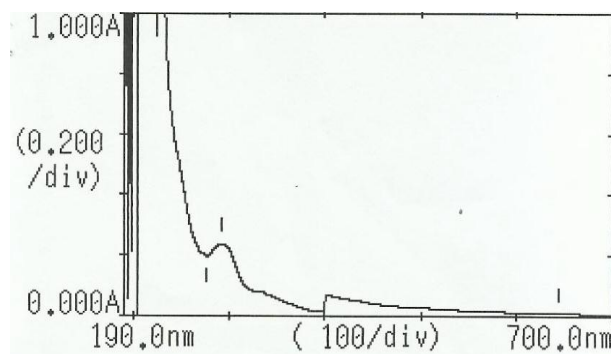
Fig.3: Sodium methoxide spectrum of compound I
