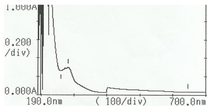
Fig.6: Boric acid spectrum of compound I
