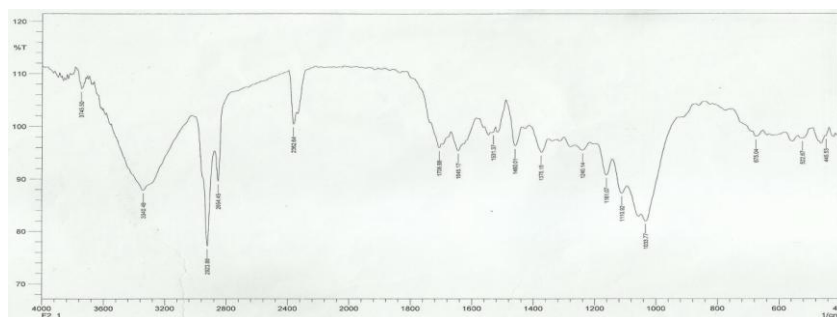
Fig.1: IR spectrum of compound I
