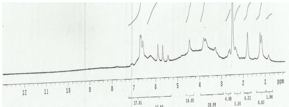
Fig.7: ^1\text{H} NMR spectrum of compound I
