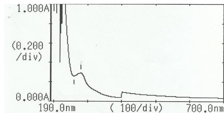
Fig.5: Aluminium chloride spectrum of compound I
