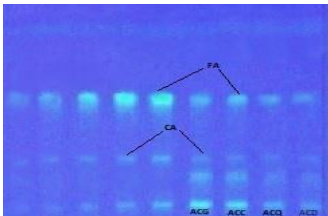
Figure 4: HPTLC plate of FA and CA at 366 nm
