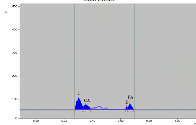
Figure 8: HPTLC chromatogram of Ananas cosmosus var Charlotte Rothschild extract
