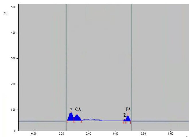
Figure 10: HPTLC chromatogram of Ananas comosus var Desi extract
