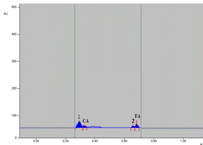
Figure 11: Overlaid spectra of standard FA and CA with four varieties of pineapple cultivar
