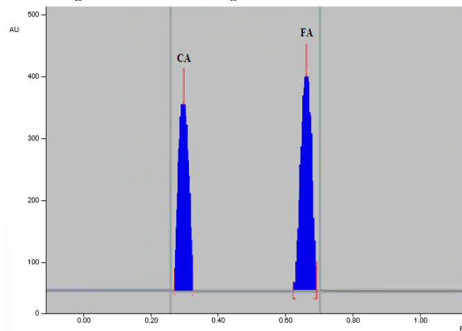
Figure 7: HPTLC chromatogram of Ananas cosmosus var Giant Kew extract
