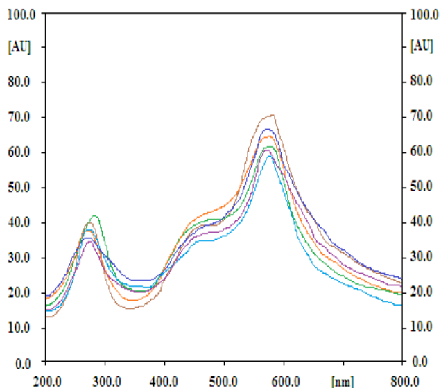
Figure 11: Overlaid spectra of standard FA and CA with four varieties of pineapple cultivar
