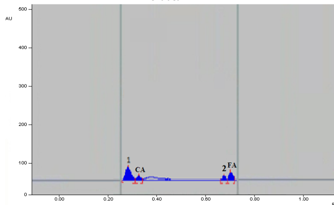
Figure 8: HPTLC chromatogram of Ananas cosmosus var Charlotte Rothschild extract
