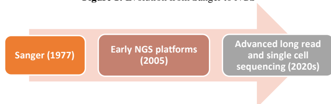
Figure 1: Evolution from Sanger to NGS
